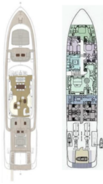
Layout Mangusta 130 Sport "SHANE"
